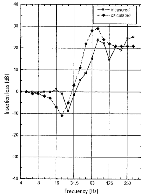
Figure 1: Measured and calculated ( M = 3000 kg, s_M'' = 0,035 N/mm 3 , ballast stiffness s_s = 5 \cdot 10^8 N/m (1+j0,5)) insertion loss of the ballast mat, type Sylomer C 340 in a rapid-transit railway tunnel near Munich.
